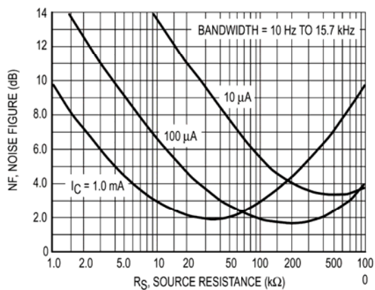
Wideband Noise Figure
