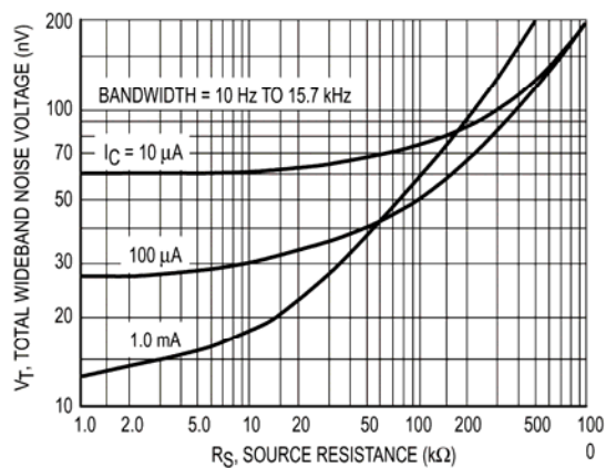
Total Wideband Noise Voltage
